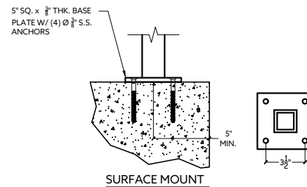
SURFACE MOUNT
