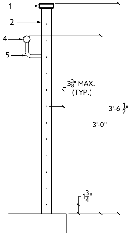
RAILING CROSS SECTION
