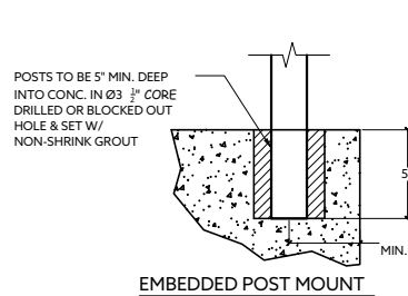
EMBEDDED POST MOUNT
