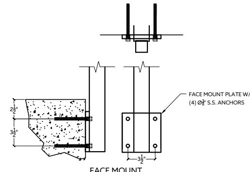
FACE MOUNT
