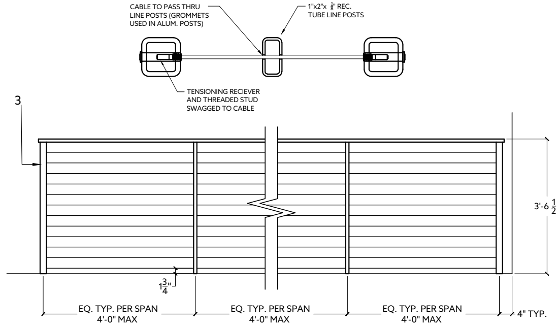
RAILING ELEVATION
