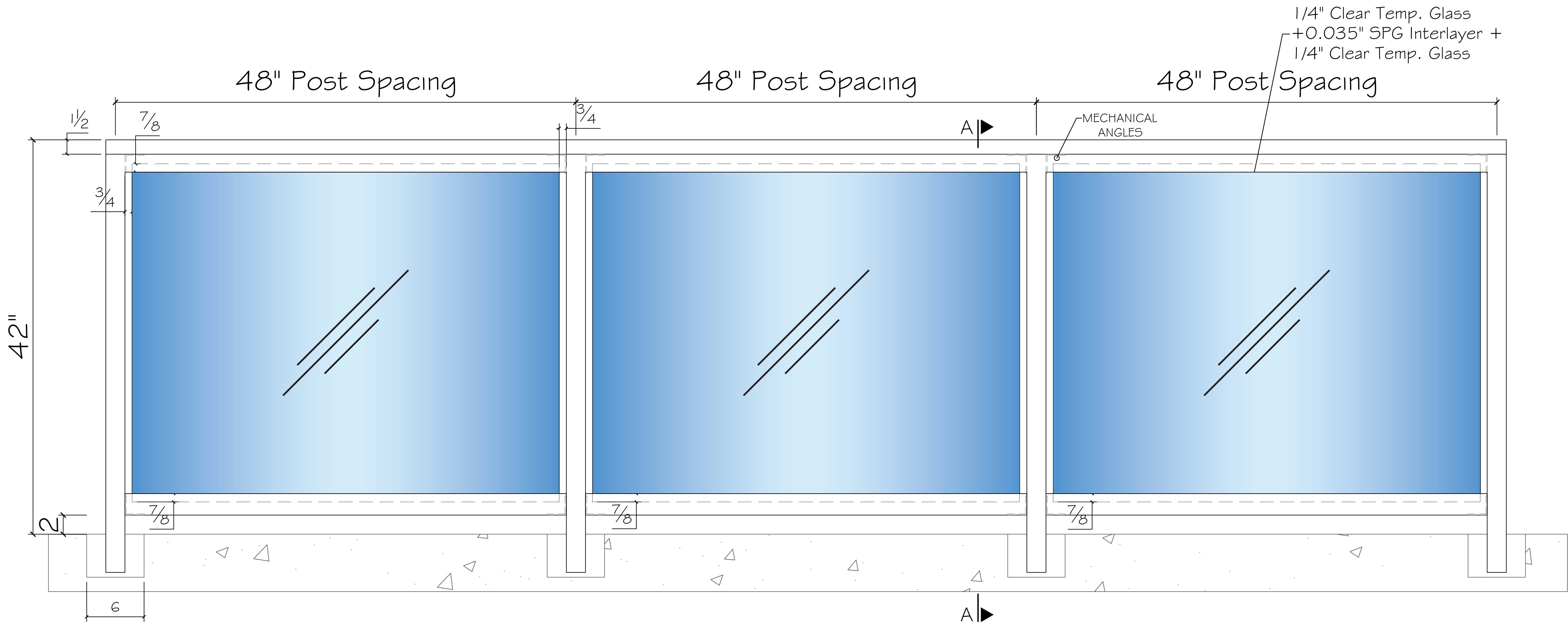
GLASS BALCONY ELEVATION Post System
